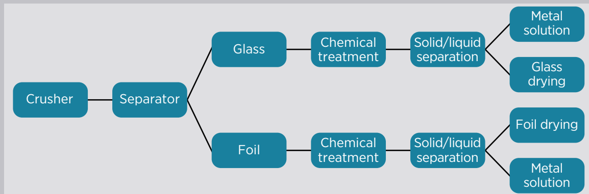
Figure 30 Losser Chemie recycling process
