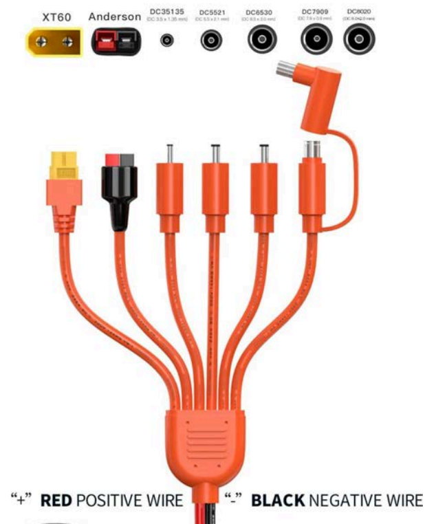
Image 7 : Various connectors
